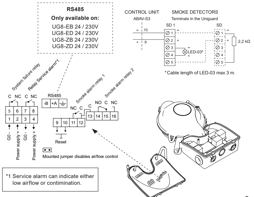
Wiring diagram: UG8-E and UG8-Z models
