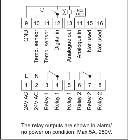
FIG. 2 (CFA-24V)
